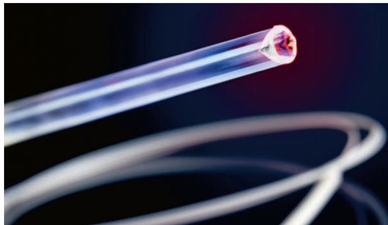
Medical glass fibre for laser treatment of vascular diseases with an inverted cone for lateral optical radiation (without cap) © Fraunhofer IZM
