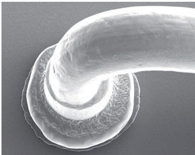
Ball bond contact on a high-strength aluminium scandium (AlSc) chip metallisation
