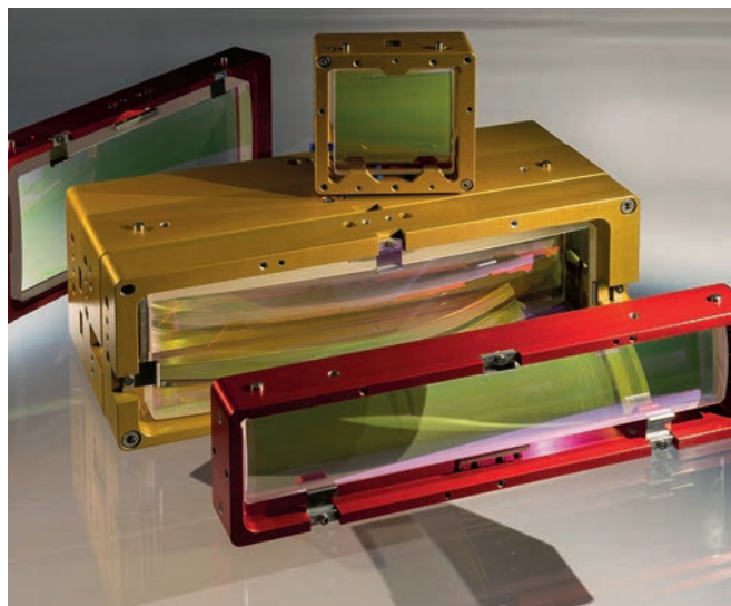
Framed optics for high-precision laser beam guidance in tension-optimised holders
