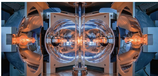
Large single crystals are produced in this optical zone melting furnace. © M. Setzpfandt/HZB
