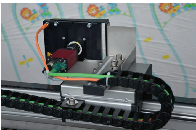
Camera on axis in front of a printing web © Bi-Ber GmbH & Co. Engineering KG
