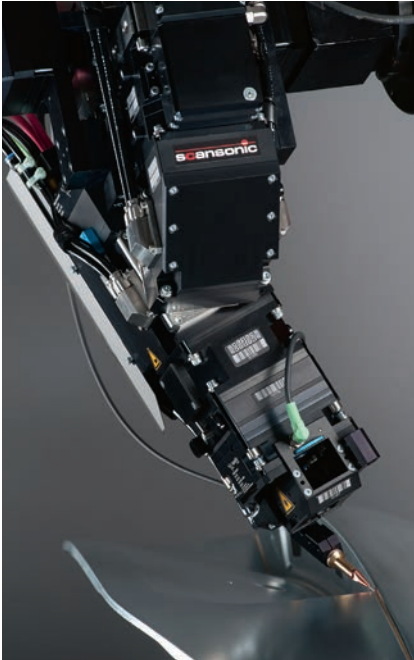
ALO3: laser processing optics with seam tracking by added wire © Scansonic Group
