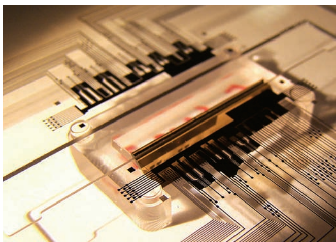
Deflecting mirror unit for optical coupling to a glass chip provided with electrical and optical waveguides for EOCB/backplane applications © Fraunhofer IZM
