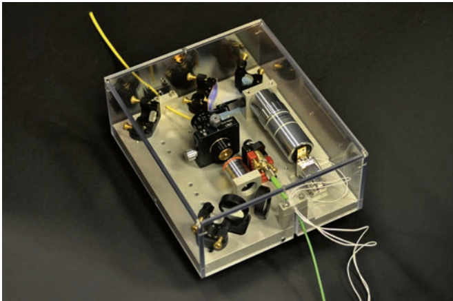
Single photon source for quantum experiments © AG Benson, HU Berlin
