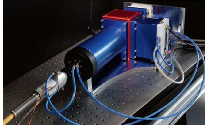
Pump module for high-energy short pulse laser systems with approx. 6 kW output power from the fibre
