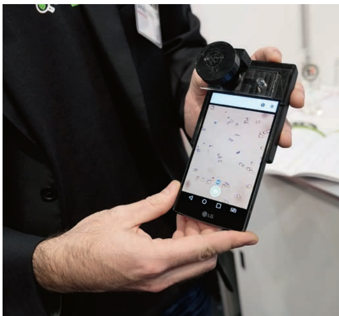
With the mobile phone microscope from Oculyze, for example, it is possible to count cells automatically. © Oculyze GmbH
