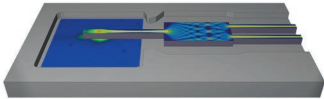
Element consisting of an integrated quantum optical chip © TU Berlin/AG Optoelektronik
