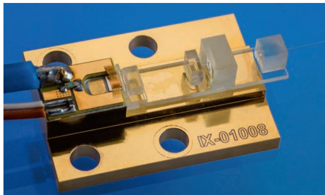
Fully glass-based micro-optical bench for compact diode laser modules with beam rotation and merging of multiple channels onto one optical fibre © Fraunhofer IZM
