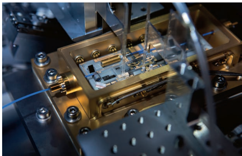
Precision assembly of a fibre-coupled diode laser module for space applications at FBH © FBH/schurian.com
