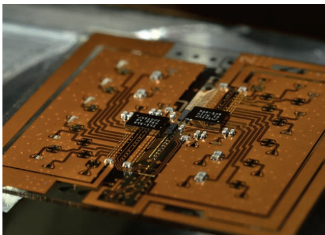
4x25 Gbps/channel on-board transceiver on glass interposer with through-hole plating and integrated lens arrays © Fraunhofer IZM
