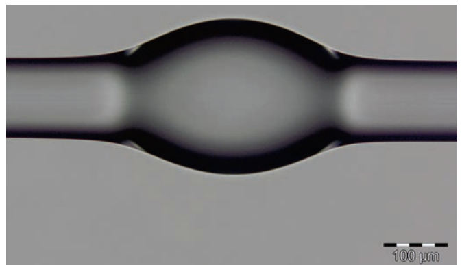
Fibre-optic resonator for optical position determination and biochemical sensor technology © Fraunhofer IZM
