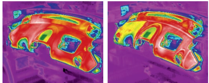
Thermographic recording of a vehicle cockpit component with identified defect (left) and after optimisation (right)
