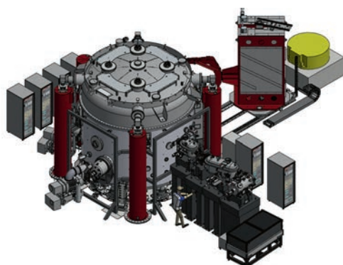
Reflectometer system for large samples (sample diameter up to 1,500 mm, total load up to 800 kg) with integrated source and monochromator beam tube for the wavelength range 6 nm to 20 nm
