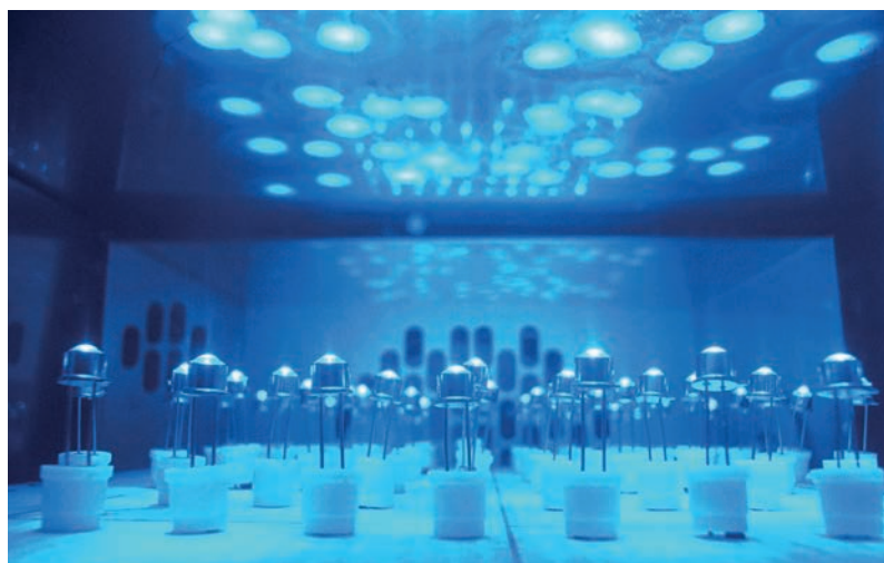
Measuring site for LEDs © Epigap Optronik GmbH
